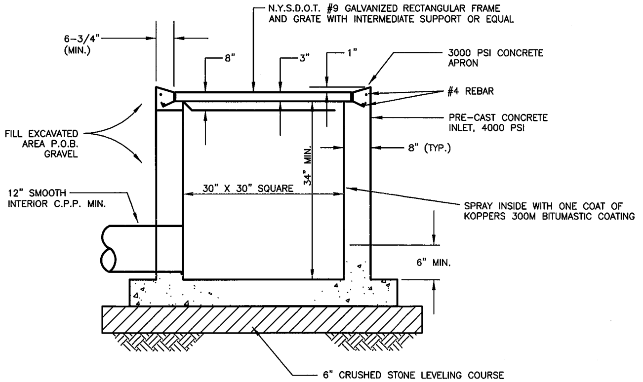
SECTION VIEW
