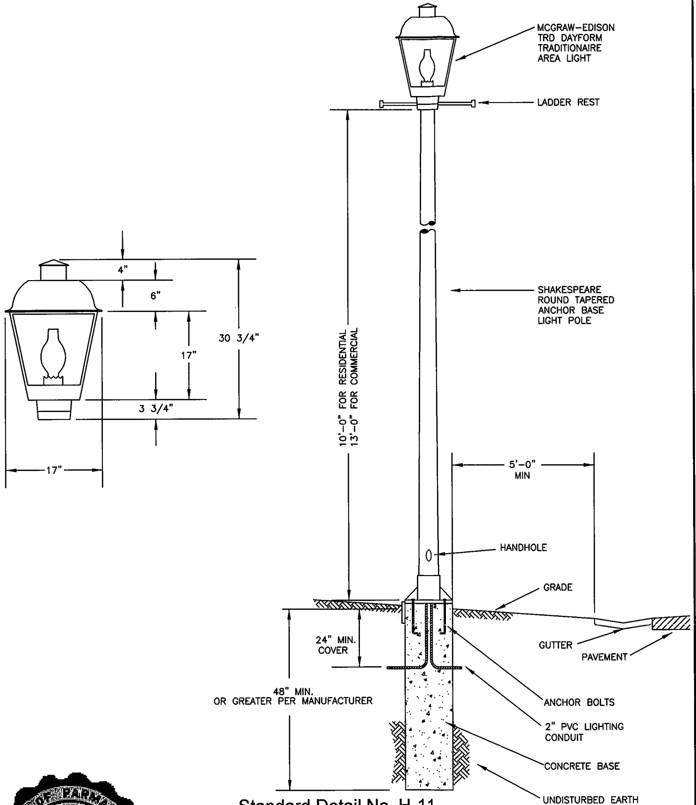
Standard Detail No. H-11 Typical Light Pole Standard Detail Scale: N.T.S.
