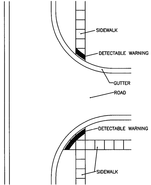
DETECTABLE WARNING AT INTERSECTIONS
